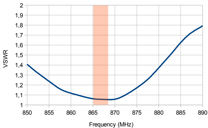
VSWR vs Frequency (MHz)
